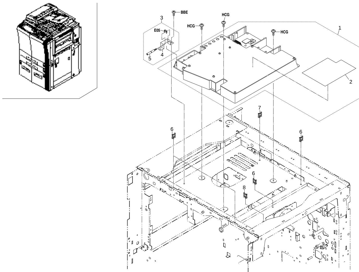
FIG. 12 LASER SCANNER UNIT
