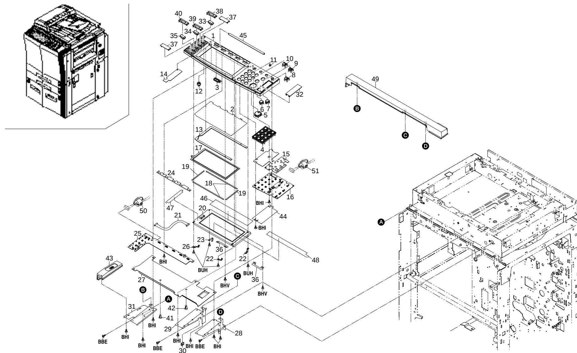
FIG. 41 OPERATION SECTION
