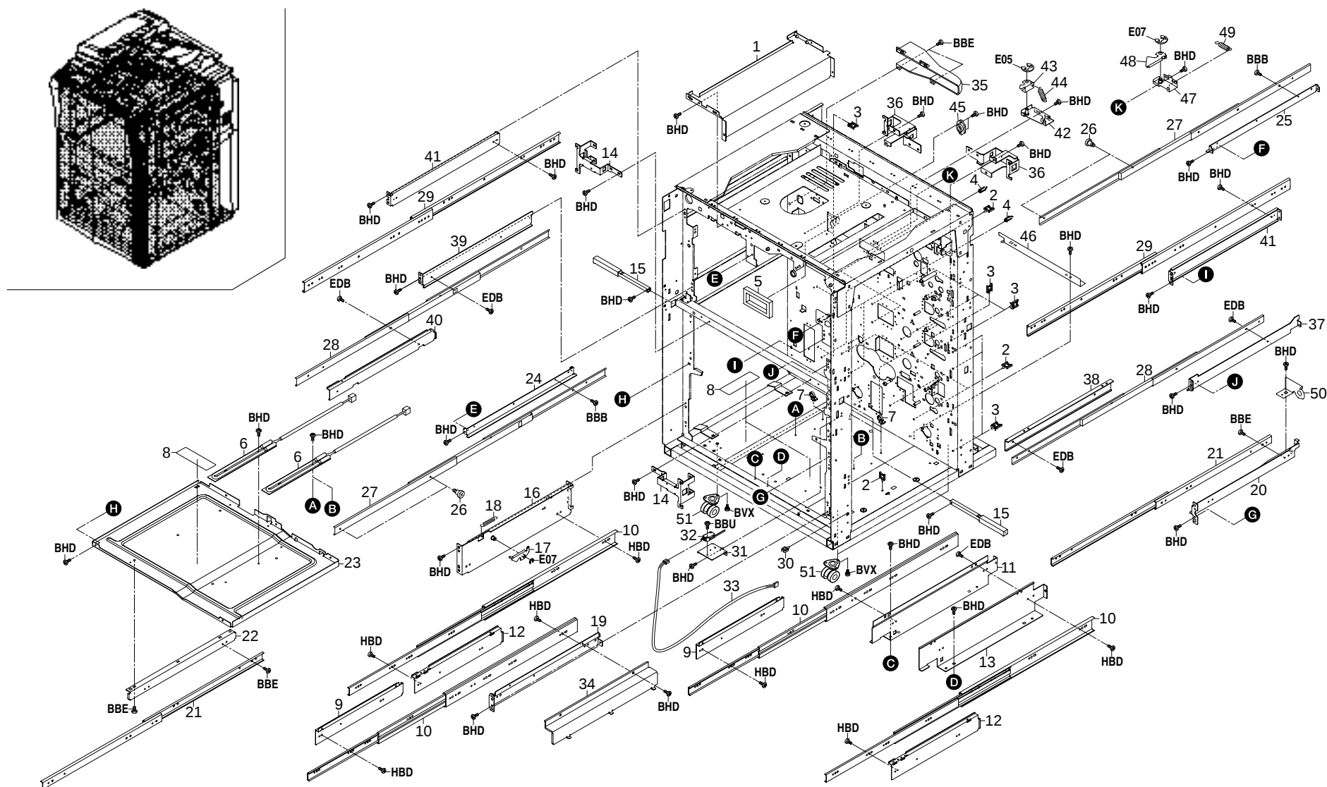
FIG. 2 FRAME SECTION
