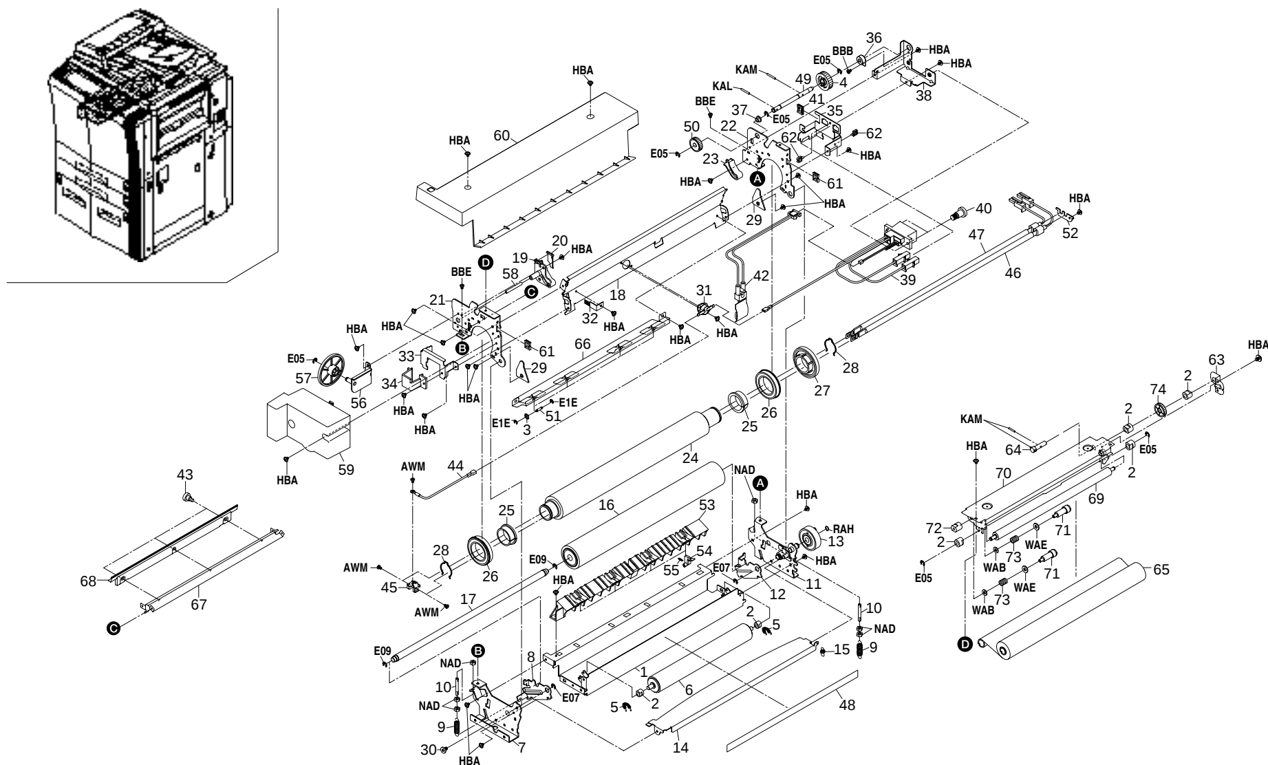
FIG. 19 FIXING SECTION
