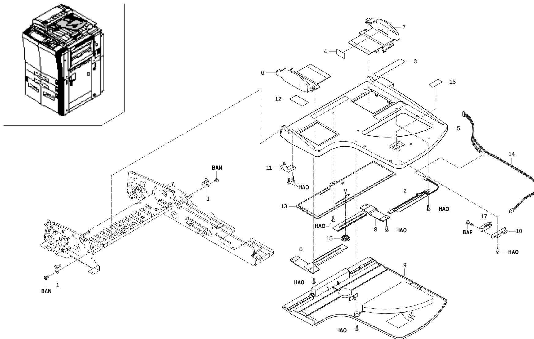
FIG. 33 PAPER FEED-IN SECTION (DF)
