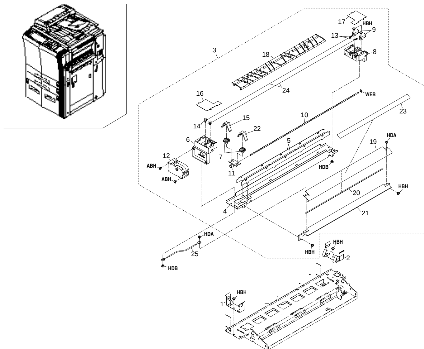
FIG. 20 TRANSFER SECTION
