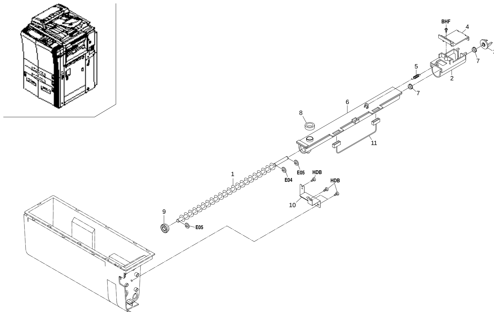
FIG. 30 HOPPER SECTION II
