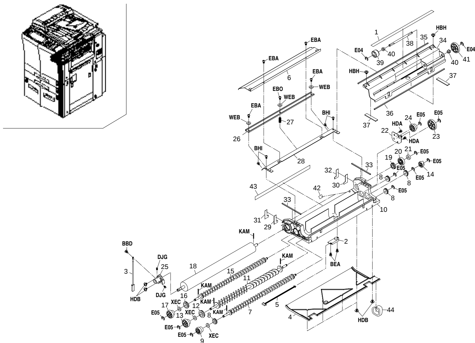
FIG. 13 DEVELOPING SECTION
