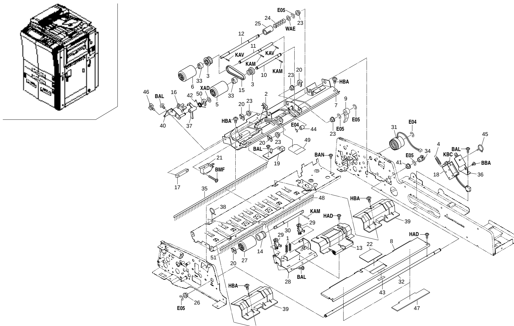
FIG. 34 PAPER CONVEYING SECTION (DF)
