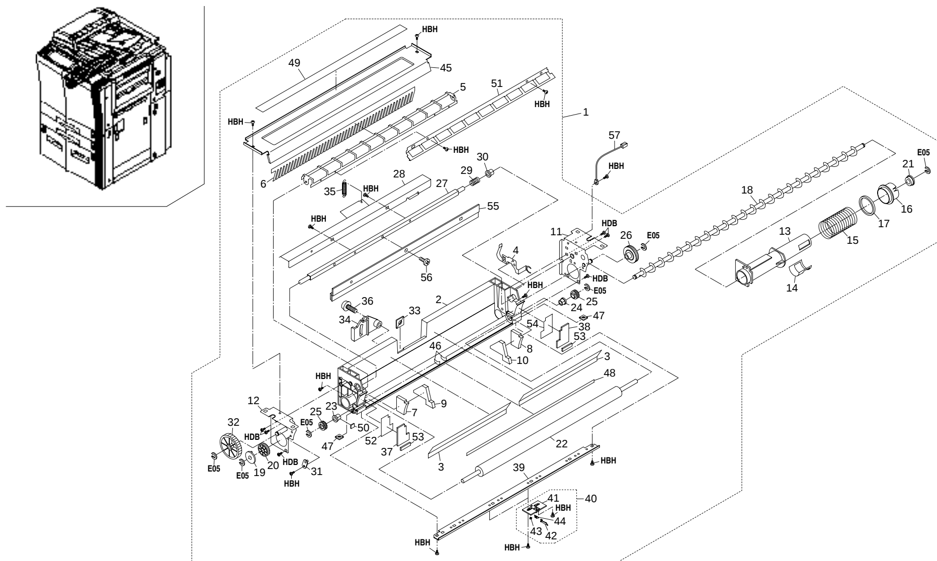
FIG. 14 CLEANING SECTION I
