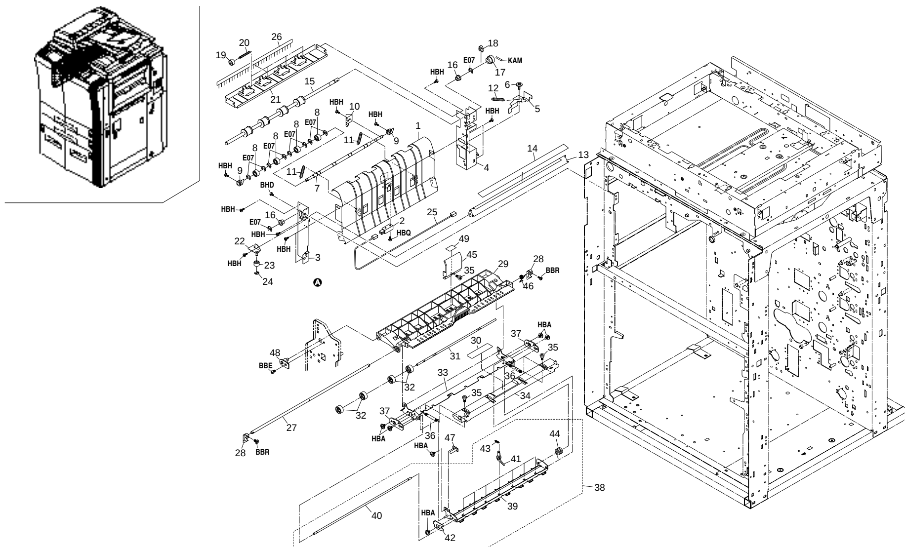
FIG. 26 EJECT SECTION
