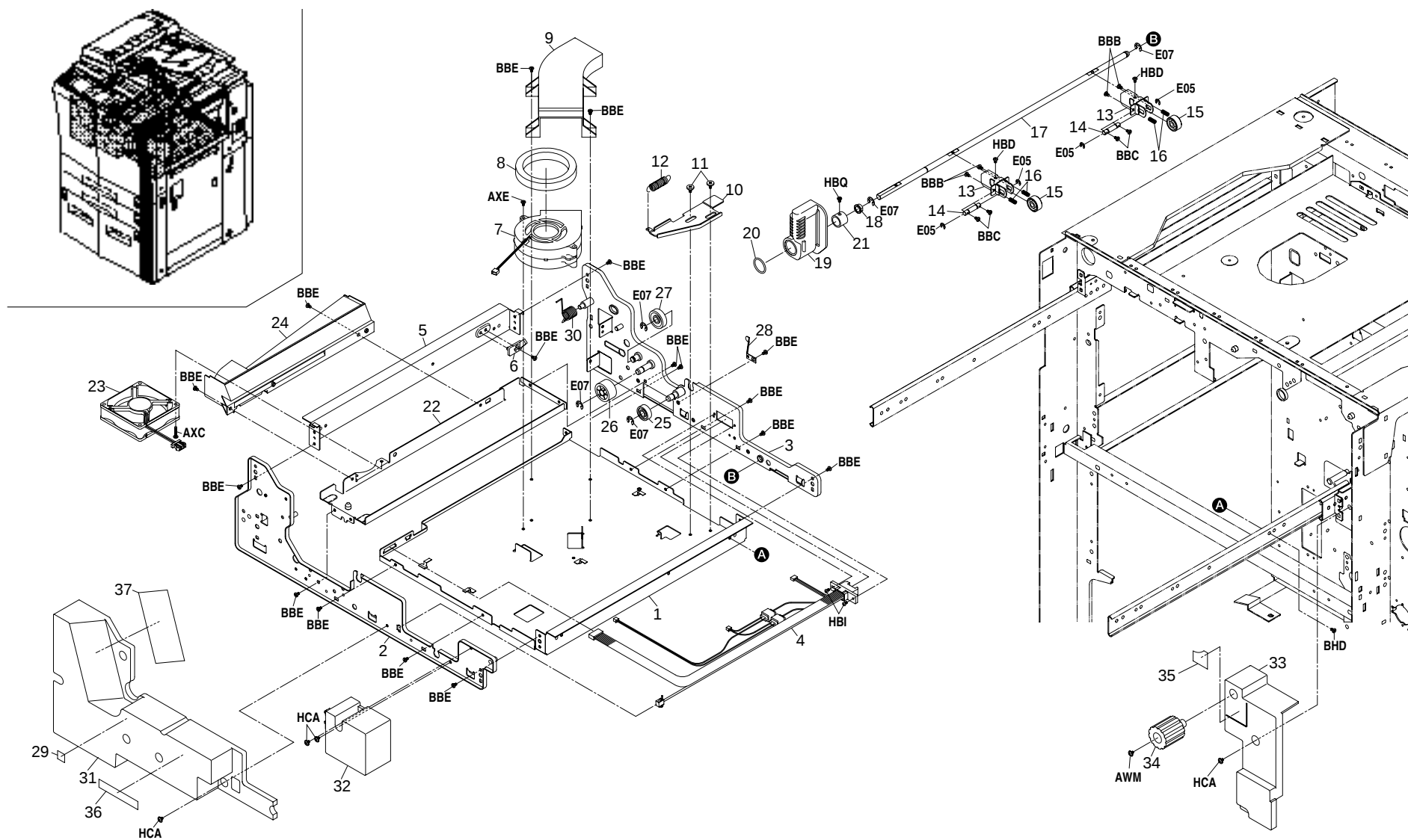
FIG. 16 CONVEYING SECTION I
